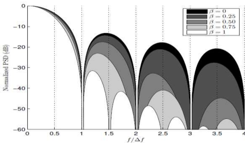
Figure 4. Rolloff effect of an OFDM subcarrier
